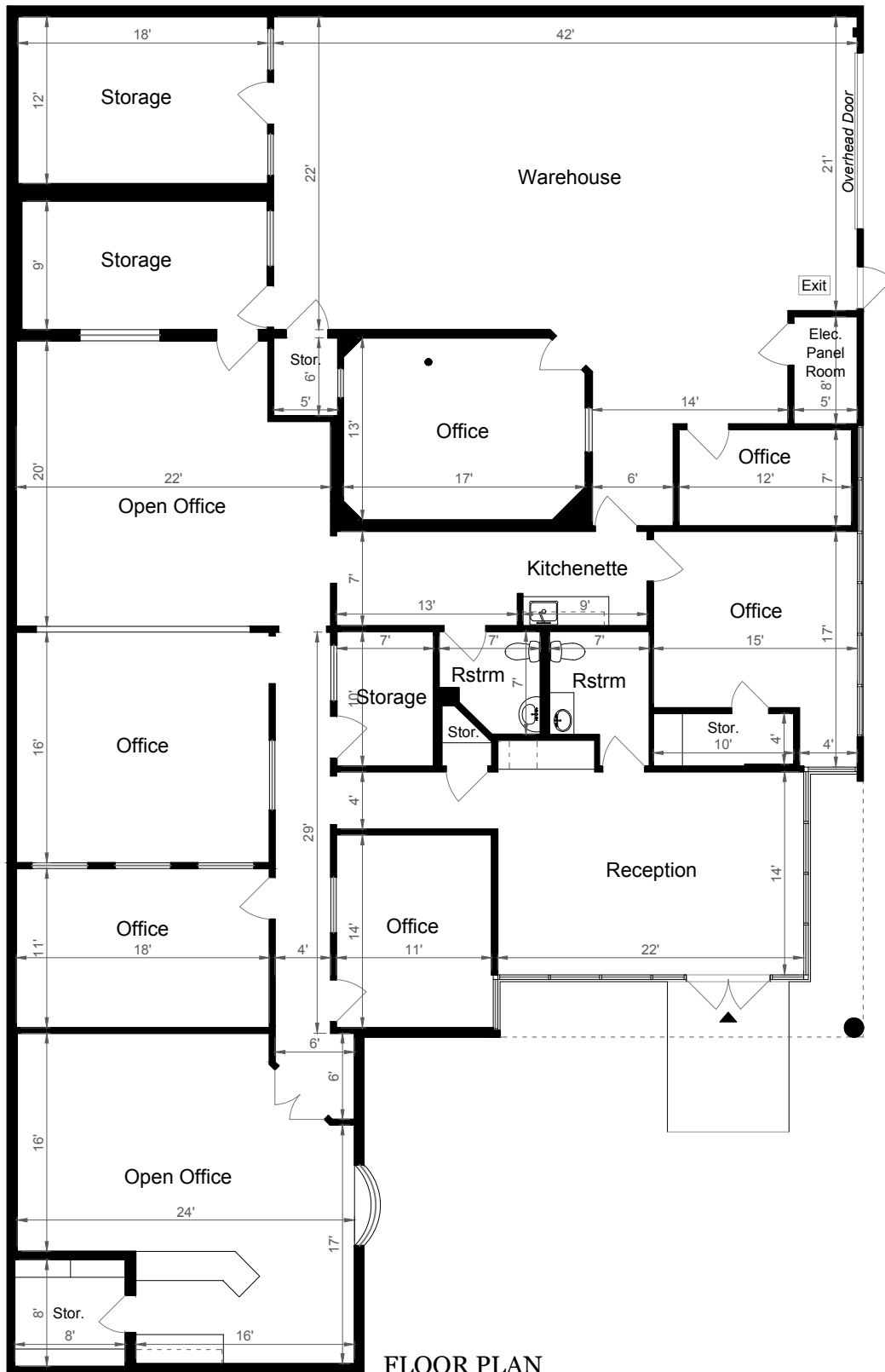
FLOOR PLAN
